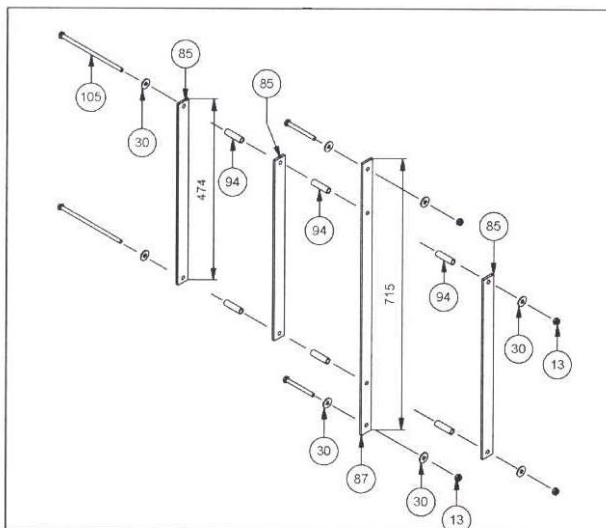
Support de tuyau S8
