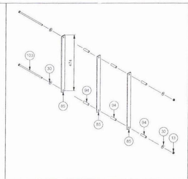
Support de tuyau S5
