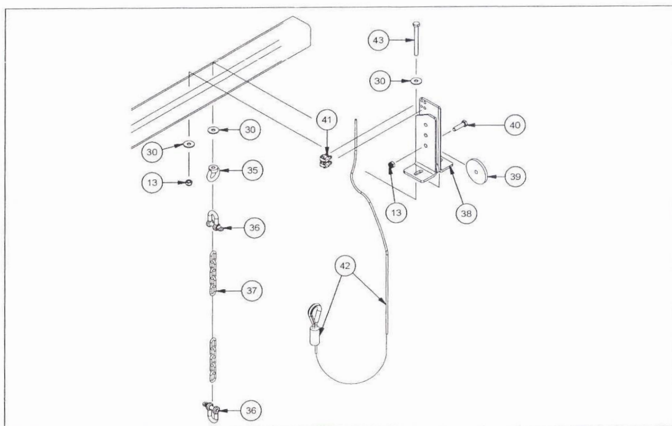
Figure H (dans figure C + figure D)
