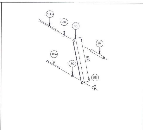
Support de tuyau S9
