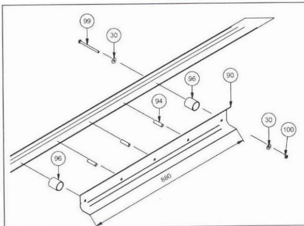
Support de tuyau S6
